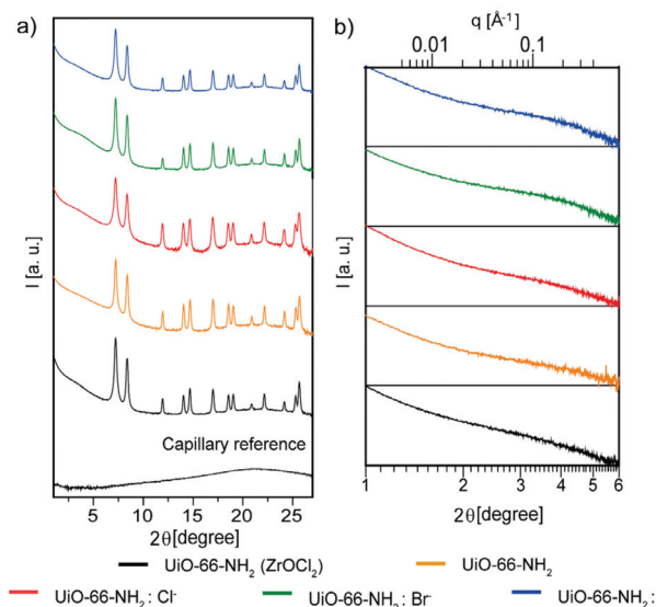
Fig. 3 Crystallographic characterization of UiO-66- NH_2 NMOFs: UiO-66- NH_2 ( ZrOCl_2 ) (black), UiO-66- NH_2 (orange), UiO-66- NH_2:Cl^- (red), UiO-66- NH_2:Br^- (green) and UiO-66- NH_2:I^- (blue). (a) WAXS analysis measured at a sample-to-detector distance of 288 mm and (b) SAXS analysis measured at a sample-to-detector distance of 1343 mm in capillary mode.
