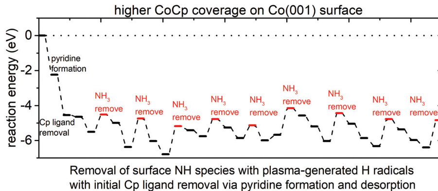
Fig. 6 The plotted reaction pathway for removal of surface NH species with plasma generated H radicals with initial Cp ligand removed from 3CoCp-terminated Co(001) surface. The steps of H radical addition are indicated by the black markers and the steps of NH 3 desorption are indicated by the red markers. The Cp ligand is first eliminated as pyridine.
