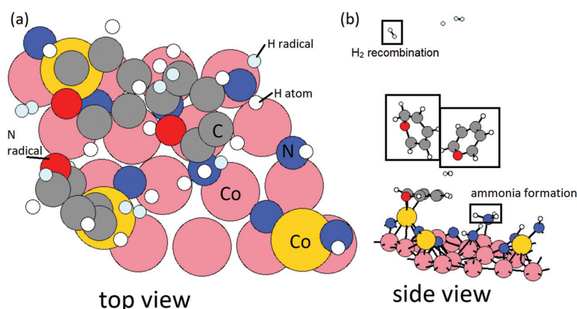
Fig. 9 The structure snapshot at the end of the MD calculation at 600 K on the \text{NH}_x -terminated Co(001) surface with 9 H radicals in (a) top view, and (b) side view. Carbon, nitrogen, and hydrogen atoms are presented in grey, blue, and white colours. H radicals are represented by light blue spheres. Substrates Co and Co from \text{CoCp}_2 are represented by pink and yellow spheres, respectively. H and N radicals are represented by light blue and red spheres, respectively.
