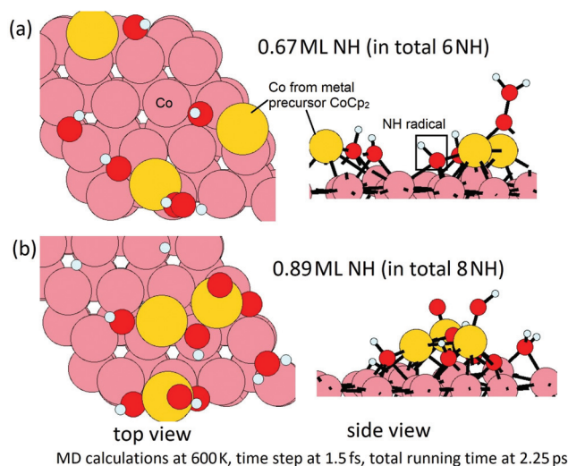
Fig. 12 The configurations of the structures after MD calculations on the Co(001) surface with NH radicals at the coverage of (a) 0.67 ML, and (b) 0.89 ML. Carbon, nitrogen, and hydrogen atoms are presented in grey, blue, and white colours. Substrates Co and Co from \text{CoCp}_2 are represented by pink and yellow spheres, respectively. Plasma-generated N and H radicals are represented by red and light blue spheres, respectively.
