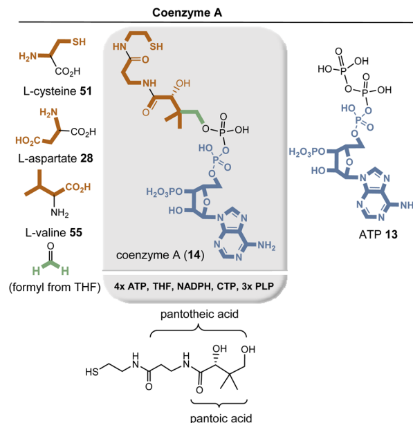
Fig. 18 Summary of coenzyme A (14) biosynthesis: building blocks are marked in sienna, blue and green at positions where they end up in coenzyme A. Coenzyme-dependent enzymes: ATP: PanA, CoaD, CoaE; CTP: CoaB; THF: ketopantoate hydroxymethyltransferase (PanB); NADPH: ketopantoate reductase (PanE); PLP: aspartate 1-decarboxylase (PanD), 4'-phosphopantothienoyl cysteine decarboxylase (CoaC) and valine-pyruvate transaminase.
