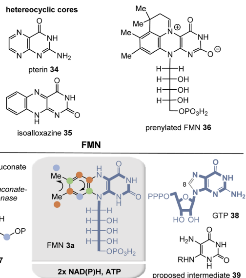
Fig. 4 Structures of pterin 34, isoalloxazine 35 and prFMN 36 (top). Summary of flavin biosynthesis with building blocks marked in sienna and blue including positions where they end up (bottom). Coenzyme-dependent enzymes: \text{NAD(P)H} : 6-phosphogluconate-dehydrogenase and 5-amino-6-(5-phosphoribosylamino)uracil reductase ( ribD ); ATP: riboflavin kinase ( ribF ); biosyntheses in fungi and bacteria only differ in timing of individual steps.
