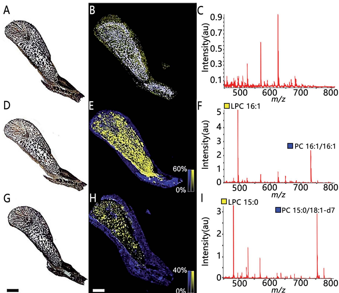
Fig. 5 The use of functional MSI to study phospholipase A2 activity against two different lipid substrates, PC 16:1/16:1 and PC 15:0/18:1-d7, from N. subfulva venom gland. Optical images of venom gland tissue sections in the absence of lipid substrate (A), the addition of the substrate phosphatidylcholine (PC) 16:1/16:1 (D) and a deuterium-labeled substrate PC 15:0/18:1-d7 (G). (B, E and H) MALDI images of the substrate (blue) and their corresponding PLA2 product (yellow) for each section. (C, F and I) Averaged MALDI mass spectra in the absence of lipid substrate and addition of the two substrates. Scale bar, 2 mm. Sample sections were coated with \alpha -cyano-4-hydroxycinnamic acid (CHCA) and measured with MALDI imaging in positive ion mode (80 \mu m raster size). Reprinted (adapted) from Hamilton et al. (2020) 35 with permission.
