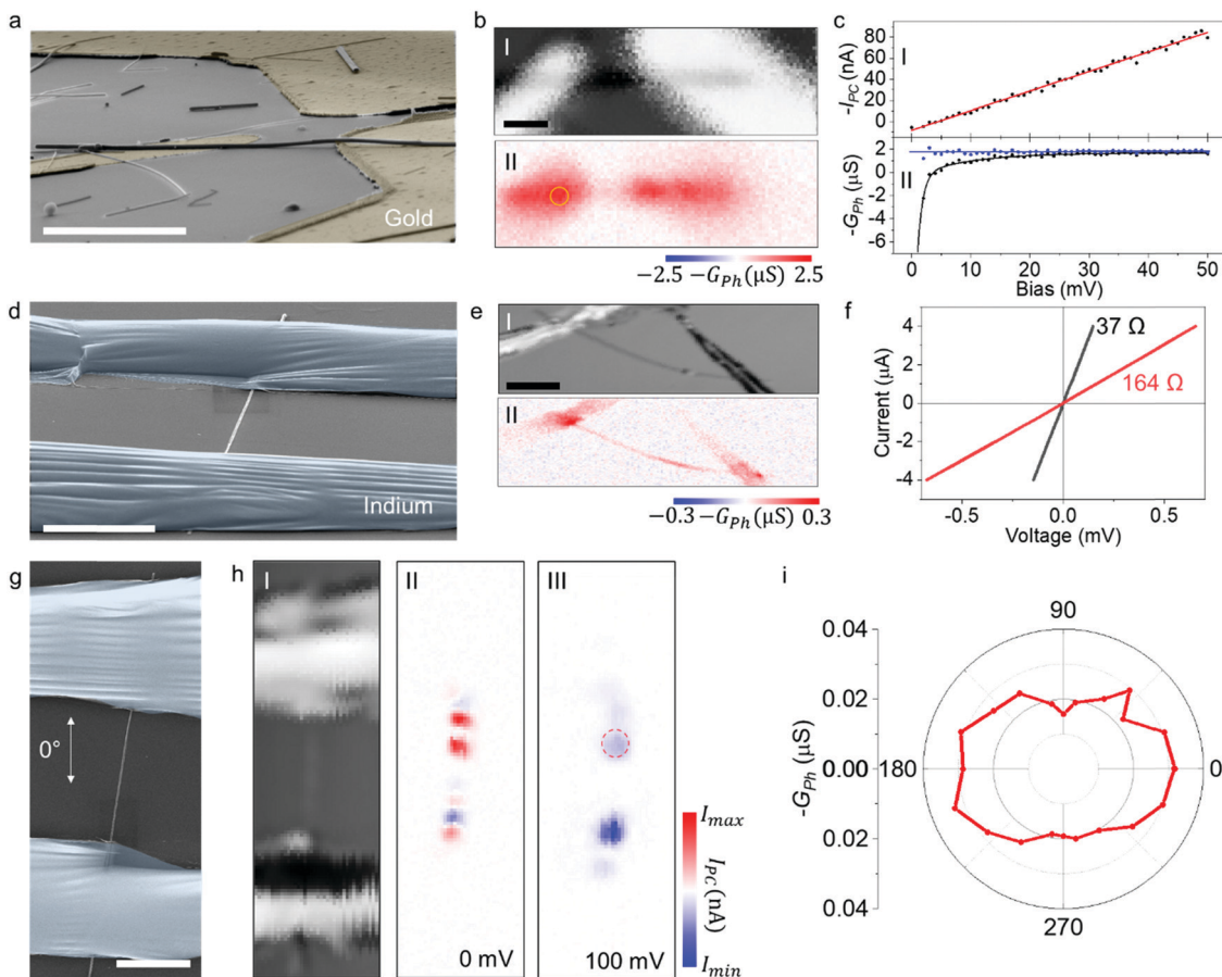
Fig. 3 (a) False colored SEM image of a Ag NW on pre-patterned gold electrodes. Scale bar is 5 μm. (b) Reflection map (I) and the corresponding -G_{Ph} map under 20 mV bias (II) showing the photoconductance over the device. It is noteworthy that there is a significant conductance modulation over the gold electrodes. A 532 nm laser source was used at 65 μW power. The yellow circle indicates the position where -I_{PC} vs. bias measurements were taken from. The scale bar is 5 μm. (c) -I_{PC} vs. bias (I) graph showing a linearly increasing -I_{PC} with the bias (black dots). The red line is the linear fit to the data. Zero bias response is \sim 6 nA. Lower panel (II) shows -G_{Ph} (black dots) and -\frac{I_{PC} - I_{PC}^0}{V} (blue dots) vs. bias. Solid lines are fits to the data. (d) False colored SEM image of an indium contacted Ag NW. Note the grating-like structures over the indium, which naturally occur due to thermal contraction upon cooling. Scale bar is 5 μm. (e) Reflection map (I) and the corresponding -G_{Ph} map under 100 mV bias (II) showing the conductance modulation over the indium contacts. Notice that the modulation intensifies near the indium-NW junction. Also, the visible defect in the reflection map results in enhanced plasmonic response, which is clear in the photoconductance map. Data were collected with a 532 nm laser at 96 μW. Scale bar is 10 μm. (f) Current vs. voltage graphs of the same devices, before (red dots) and after (black dots) reduction of the photoconductance. (g) False colored SEM image of a device with the incident polarization angle marked. (h) (I) Reflection map, (II) open-circuit response, and (III) 100 mV response maps are shown. I_{max} = 0.25 nA for (II), 25 nA for (III) and I_{min} = -0.25 nA for (II) and -25 nA for (III). (i) The polar chart shows the incident polarization angle vs. -G_{Ph} at 100 mV bias. The data were collected from the individual maps taken around the red dashed circle in h (III).
