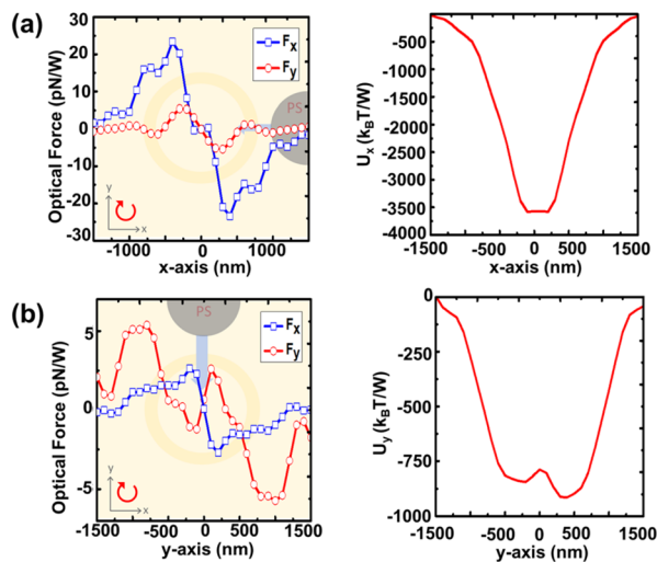
Fig. 8 Calculated optical performances of PVL 2-arms with a CG using a 1 \mu\text{m} PS bead. Rotating force ( F_x , F_y ) and rotating potential U along the (a) x-axis and (b) y-axis under LCP illumination.
