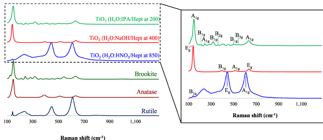
Fig. 3 (Left) Raman spectra overlay of simulated rutile (navy blue), anatase (dark red), and brookite (dark green) phases, as well as the Raman spectra of the TiO 2 particles synthesized through the PIT-nano-emulsion method, employing H 2 O : HNO 3 /heptane (blue), H 2 O : NaOH/heptane (red), and H 2 O : IPA/heptane (green) emulsion systems and after thermal treatment. (Right) Raman spectra for TiO 2 particles under each condition with the prominent Raman modes identified.
