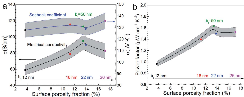
Fig. 8 (a) The electrical conductivity \sigma and the Seebeck coefficient \alpha and (b) power factor \alpha^2\sigma of nanporous \text{Ca}_3\text{Co}_4\text{O}_9 films as function of surface porosity fraction at room temperature.
