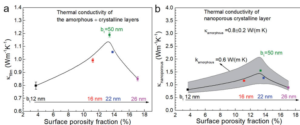
Fig. 9 (a) Effective thermal conductivity \kappa_{\text{film}} of \text{Ca}_3\text{Co}_4\text{O}_9 films as a function of surface porosity fraction, and (b) thermal conductivity of the nanporous crystalline \text{Ca}_3\text{Co}_4\text{O}_9 layer \kappa_{\text{nanoporouse}} , assuming \kappa_{\text{amorphous}} = 0.8 \text{ W m}^{-1} \text{K}^{-1} with a \pm 0.2 \text{ W m}^{-1} \text{K}^{-1} uncertainty captured by error bars.
