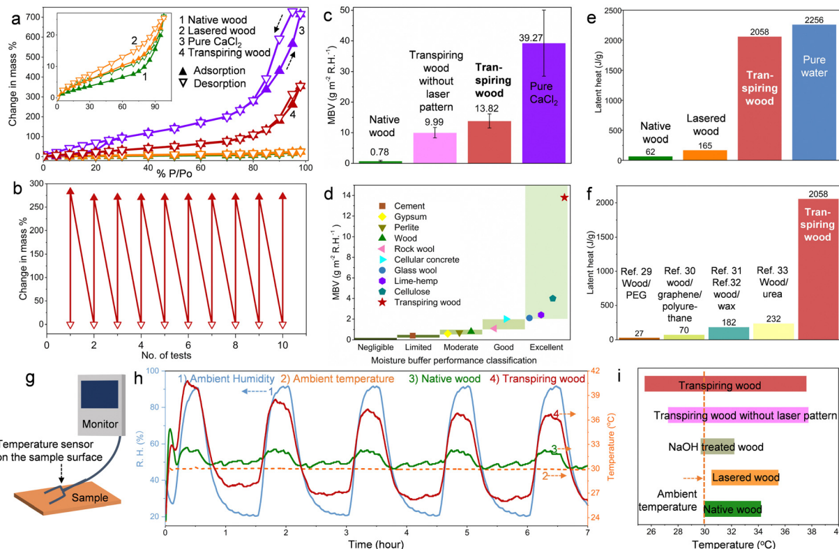
Fig. 2 Moisture sorption performance of transpiring wood at the material level. (a) Water sorption isotherms of native wood, lasered wood, \text{CaCl}_2 powder, and transpiring wood at 25 °C. (b) Water-uptake profile swung between 0–98% R.H. for ten cycles. (c) Moisture buffer value of native wood, wood- \text{CaCl}_2 composite (without lasered pores), \text{CaCl}_2 powder, and transpiring wood. (d) Moisture buffer performance classification of common building materials and transpiring wood. (e) Calculated latent heat of water-saturated samples from isothermal differential scanning calorimetry (DSC). (f) Comparison of the latent heat of transpiring wood with that of previously reported wood-phase change material composites. (g) An illustration showing the set-up of monitoring the materials' surface temperature during the water sorption/desorption. (h) Surface temperature changes of native and transpiring wood resulting from the exposure to dynamic humidity swings (between 20% and 90% R.H.) at 30 °C ambient temperature. (i) The range of surface temperature change of transpiring wood compared to its precursors.
