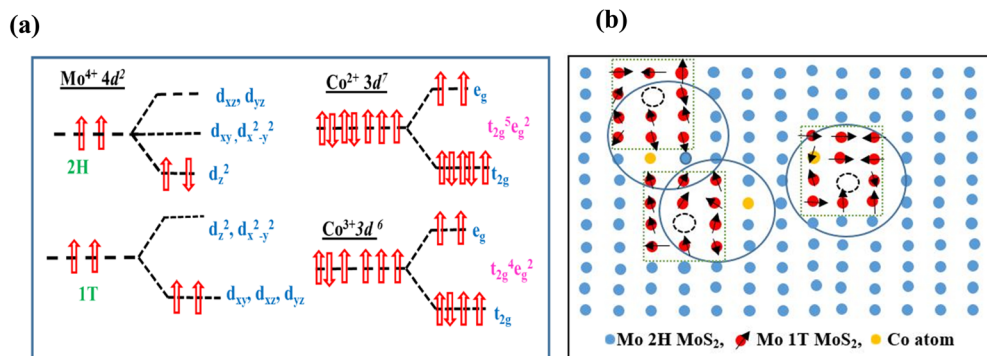
Fig. 10 (a) Electron orbital degenerate states of Mo atoms ( \text{Mo}^{4+} ionic state) in 1T and 2H configuration and Co atoms ( \text{Co}^{2+} and \text{Co}^{3+} ionic state). (b) Schematic representation of the bound magnetic polaron model mediated by vacancy and Co dopant in \text{MoS}_2 NFs. 1T phases are induced around vacancy and Co atom forming spin polarized states.
