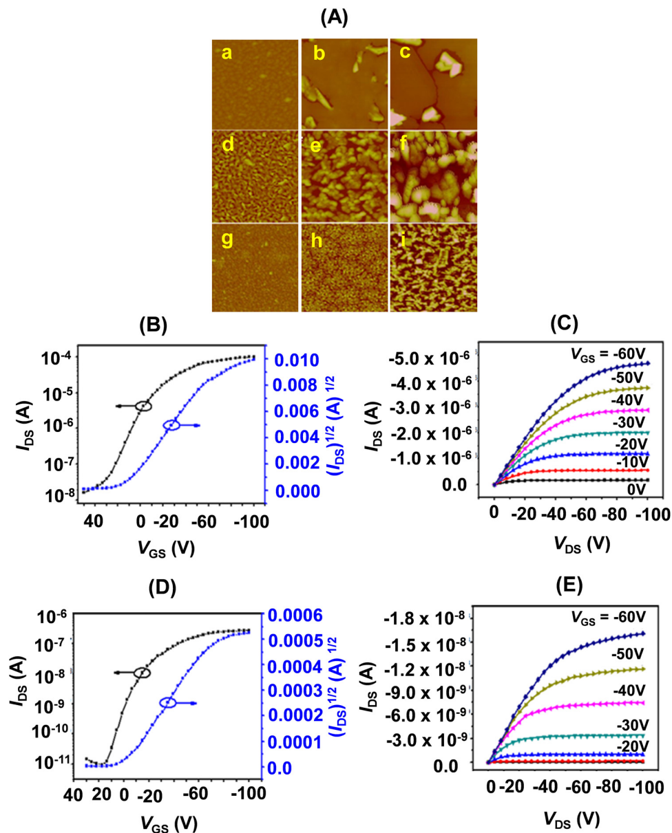
Fig. 9 (A) AFM images ( 5 \times 5 \mu\text{m} ) of 50 nm thick films of 22f–h , (a, d and g) T_s = 25 \text{ }^\circ\text{C} ; (b, e and h) T_s = 60 \text{ }^\circ\text{C} ; (c, f and i) T_s = 100 \text{ }^\circ\text{C} . (B/D) Transfer and (C/E) output characteristics of the thin film OFET devices of 22f/22g (deposited on OTS treated \text{SiO}_2/\text{Si} substrate ( T_s = 25 \text{ }^\circ\text{C} )). Reproduced with permission from ref. 19. Copyright 2014, The Royal Society of Chemistry.
