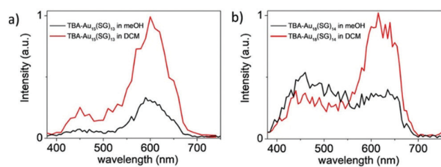
Fig. 15 Two-photon excited fluorescence spectra for (a) TBA- \text{Au}_{15}(\text{SG})_{13} and (b) TBA- \text{Au}_{18}(\text{SG})_{14} at the excitation wavelength of 780 nm. Reproduced with permission. 180 Copyright 2018. Wiley-VCH.
