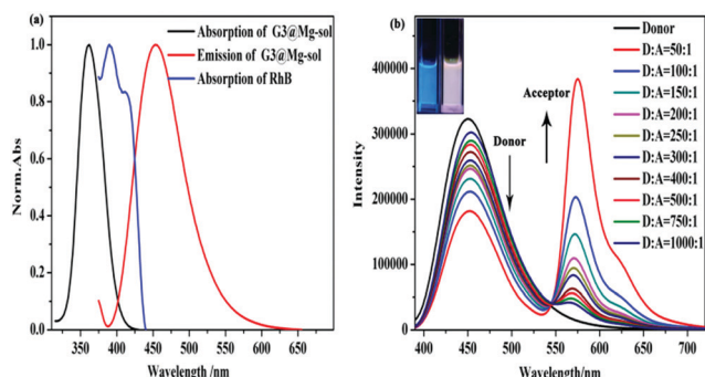
Fig. 2 (a) Normalized absorption and emission spectrum of G3@Mg-sol, and absorption spectrum of RhB. (b) Fluorescence spectrum of G3@Mg-sol/RhB ([G3@Mg-sol] = 1 \mu\text{M} , [RhB] = 0.02 \mu\text{M} ) in ethanol and water with different concentrations of RhB (Inset: photographs of G3@Mg-sol and G3@Mg-sol/RhB).
