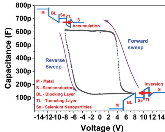
Fig. 5 Capacitance–voltage behavior of selenium nanoparticle-based charge storage memory device. Arrows show the sequence of the measurement. Trapping and de-trapping of charges in the accumulation and inversion region, respectively, have been detailed in the illustration.
