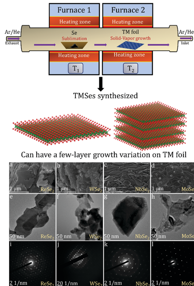
Fig. 7 Schematic of the furnace with the direction of Se vapor flow in the setup as photographed in Fig. 6 (the setup was used to synthesize ReSe_2 , WSe_2 , NbSe_2 , and MoSe_2 from the respective transition metal foils as per a previous solid-vapor CVD growth approach in the Nessim Lab). Fig. 6 shows the initiation of primary and secondary surface nucleation during CVD synthesis of layered TMSes on the transition metal foil depicted in blue. (a), (b), (c), and (d) denote high-resolution scanning electron microscopy (HRSEM) images of few-layered ReSe_2 , WSe_2 , NbSe_2 , and MoSe_2 ; (e), (f), (g), and (h) denote low magnification transmission electron microscopy (TEM) images of ReSe_2 , WSe_2 , NbSe_2 , and MoSe_2 ; (i), (j), (k), and (l) denote the selected area diffraction (SAED) pattern of ReSe_2 , WSe_2 , NbSe_2 , and MoSe_2 , indicating that they are of a single-phase. The bulk and exfoliated images are conclusive towards the layered morphology of TMSes being prepared by the ambient pressure CVD. Each material was thoroughly optimized with respect to reaction parameters to convert the transition metal foil to the corresponding TMSe fully. Therefore, such CVD-based reactions are highly scalable, providing a better yield of the layered TMSes.
