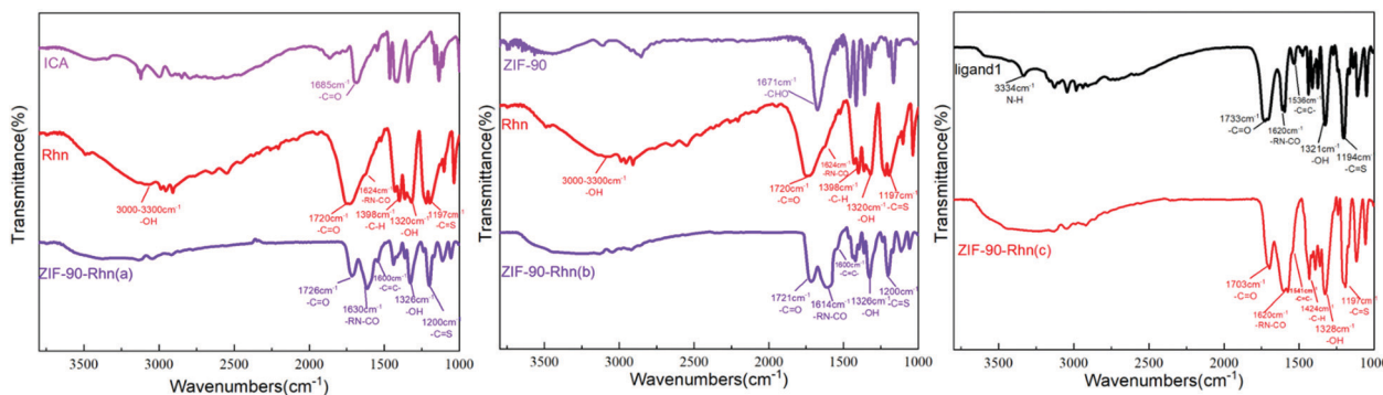
Fig. 2 FT-IR spectra of ZIF-90-Rhn(a-c) and relative compounds (on the left: ZIF-90-Rhn(a) and relative compounds; the middle figure: ZIF-90-Rhn(b) and relative compounds; on the right: ZIF-90-Rhn(c) and relative compounds).
