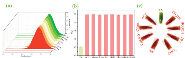
Fig. 9 (a) Fluorescence intensity of ZIF-90-Rhn@Ag + /Cy-N in ethanol (100 μM/100 μM) in different analytes (FA, acetaldehyde (ACE), trichloroacetaldehyde (Chloral), acetamide (C 2 H 5 NO), acrylonitrile (AN), trichloromethane (CH 3 Cl), diethanolamine (DEA), formic acid (HCOOH), methanol (CH 3 OH), 25 μM respectively). (b) R/G values of ZIF-90-Rhn@Ag + /Cy-N in ethanol (100 μM/100 μM) with different analytes. (c) The color changes of ZIF-90-Rhn@Ag + /Cy-N in ethanol (100 μM/100 μM) in different analytes. \lambda_{\text{ex}} = 678 \text{ nm} , \lambda_{\text{em}} = 722 \text{ nm} .
