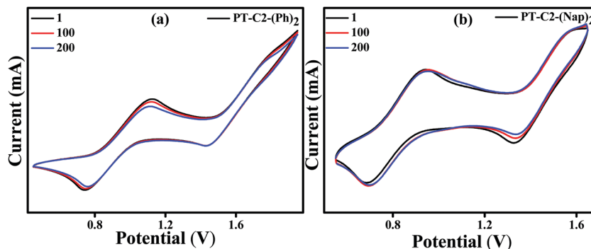
Fig. 4 Cyclic voltammograms (200 mV s -1 ) of PT-C2-(Ph) 2 (a) and PT-C2-(Nap) 2 (b) (1st, 100th and 200th cycles) in DCM (ca. 1.0 mM) recorded in CH 2 Cl 2 using TBAPF 6 (0.1 M) as the supporting electrolyte.
