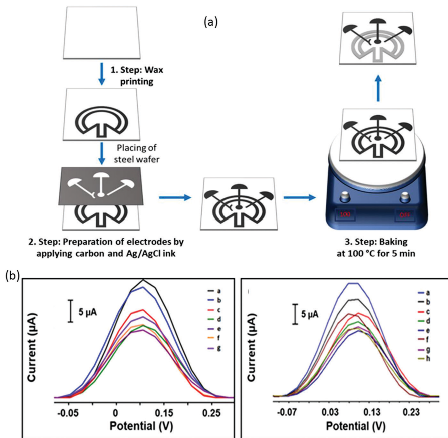
Fig. 6 (a) Steps involved in the fabrication of paper-based sensor for detection of microRNAs (b) Voltammograms in the absence of microRNAs. Source: reprinted from H. Torul, E. Yari, E. Eksin, A. Ganguly, J. Benson, U. Tamer, et al. , Paper-Based Electrochemical Biosensors for Voltammetric Detection of miRNA Biomarkers Using Reduced Graphene Oxide or MoS 2 Nanosheets Decorated with Gold Nanoparticle Electrodes, Biosensors. , 2021, 11 (7), 236.
