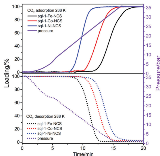
Fig. 4 Kinetics of CO 2 adsorption (top) and desorption (bottom) for sql-1-M-NCS ( M = \text{Fe, Co and Ni} ) at 288 K.
