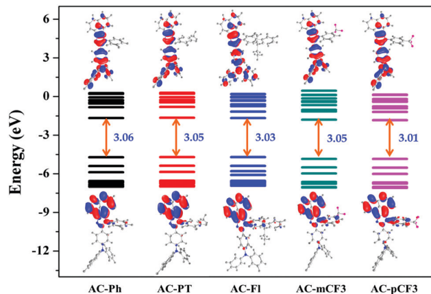
Fig. 5 Energy level diagram of AC-derivatives.
