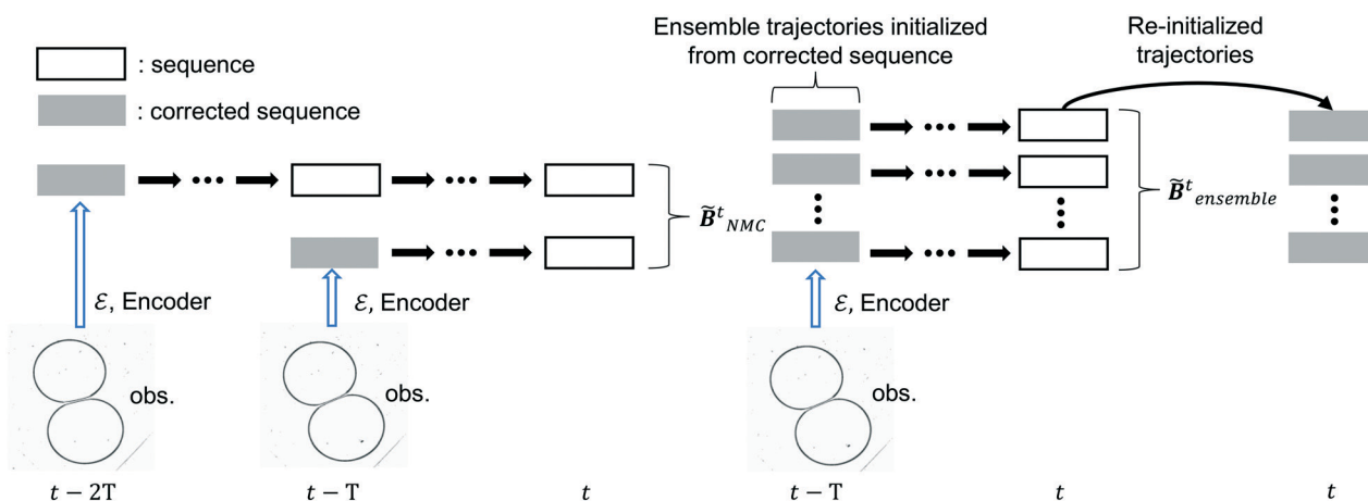
Fig. 4 Derivation of \tilde{\mathbf{B}}^t_{\text{NMC}} and \tilde{\mathbf{B}}^t_{\text{ensemble}} .
