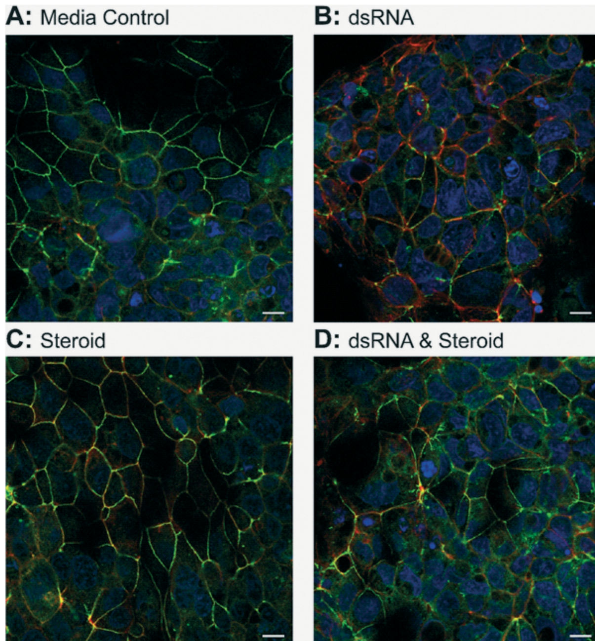
Fig. 9 Visualisation of tight junction distribution 16HBE14o- cells grown and challenged with dsRNA and corticosteroid on microfluidic chips. Images of one plane from a Z-projection stack with DAPI nuclear (blue), actin cytoskeleton (red) and occludin tight junction staining (green) for 16HBE14o- cells challenged with either media only (A), 25 \mu\text{g mL}^{-1} dsRNA (B), 100 \text{ nM} corticosteroid (C) or a combination of both dsRNA and corticosteroid (D). Z projection stack captured using confocal imaging at 63\times at wavelengths 405 \text{ nm} (DAPI), 561 \text{ nm} (actin) and 488 \text{ nm} (Occludin) (Leica TCS laser scanning microscope). White scale line indicates 10 \mu\text{m} . Data are one biological repeat in duplicate.
