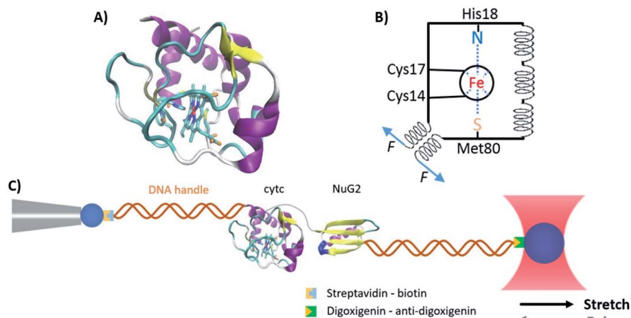
Fig. 1 The structure of horse heart cytc. (A) Three-dimensional structure of horse heart cytc (PDB code: 1hrc). Cytc is a 104 aa helical protein containing a c-type heme cofactor. The heme is covalently bound to the polypeptide chain through two thioether bonds, and the heme iron forms axial Fe–N and Fe–S coordination bonds with a histidine and a methionine residue. (B) Schematics of the structure of cytc. The black circle indicates the porphyrin ring, the spirals indicate the helices, and the blue dotted lines represent the coordination bonds. (C) Schematic of the optical tweezer experiment to investigate the mechanical unfolding–folding of cytc.
