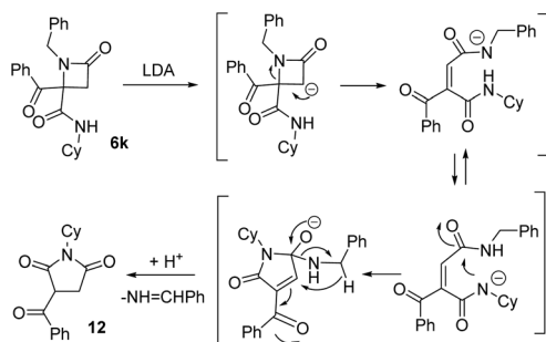
Scheme 3 Results for the treatment of azetidinone 6k with base and proposed mechanism for the synthesis of succinimide 12 (Cy = cyclohexyl).
