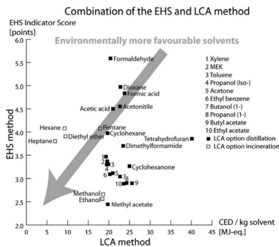
Fig. 1 Classification of 26 solvents by EHS and LCA methods representing the greenest solvents with the lowest scores. Reproduced from ref. 21 with permission from the Royal Society of Chemistry.
