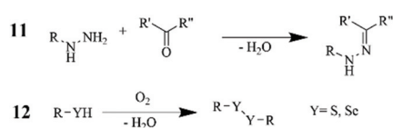
Scheme 5 Other cross-linking strategies involving hydrazone bond (11), and disulfide and diselenide formation (12).
