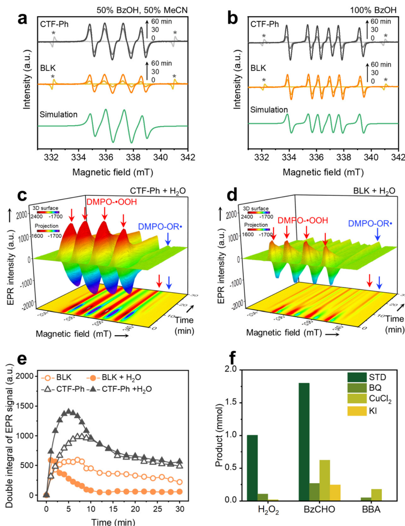
Fig. 4 Electron paramagnetic resonance (EPR) spectra of (a) DMPO-hydroperoxyl ( \text{O}_2^{\bullet-} ) and (b) DMPO-benzyl ( \text{OR}^{\bullet} ) radical with CTF-Ph and without the photocatalyst (BLK) under simulated sunlight irradiation ( \sim 980 \text{ W m}^{-2} ). Reaction conditions: (a) BzOH (1.5 mL), MeCN (1.5 mL), \text{O}_2 (purged for 30 min), 298 K, DMPO (20 \mu\text{L} ); (b) BzOH (3 mL), air (exposed to air for 3 h), 298 K, DMPO (20 \mu\text{L} ). EPR spectra were obtained at 0, 30, and 60 min of irradiation. With the photocatalyst, CTF-Ph (10 mg) was added in the reaction vessel (4 mL vial). The asterisk indicates a signal from the Mn marker used for calibration. Time-dependent in situ EPR spectra of (c) CTF-Ph and (d) BLK in an \text{O}_2 -saturated OWS (50% BzOH, 50% MeCN, 5 mol% \text{H}_2\text{O} ). (e) Double integral of the in situ EPR signals for CTF-Ph and BLK in the absence and presence of water (5 mol%) in the OWS. (f) Photocatalytic performance of CTF-Ph in the OWS with the addition of radical scavengers. Copper chloride ( \text{CuCl}_2 ), potassium iodide (KI), and 1,4-benzoquinone (BQ) were tested as photogenerated electron ( \text{e}^- ), photoinduced hole ( \text{h}^+ ), and hydroperoxyl radical ( \text{O}_2^{\bullet-} ) scavengers, respectively. Reaction conditions: CTF-Ph (20 mg), scavenger (166.7 \mu\text{mol} ), organic solution (10 mL; 50% BzOH, 50% MeCN), simulated sunlight, \text{O}_2 (1 bar), 298 K.
