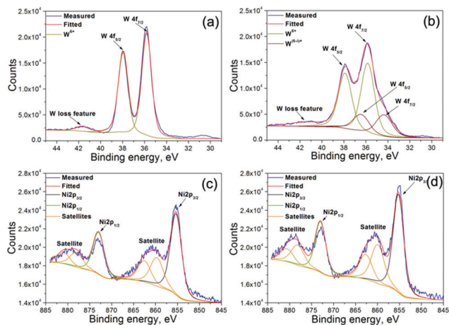
Fig. 3 XPS spectra of (a) deintercalated \text{WO}_3 , (b) intercalated \text{WO}_3 , (c) reduced \text{Ni}(\text{OH})_2 and (d) oxidized \text{Ni}(\text{OH})_2 samples.
