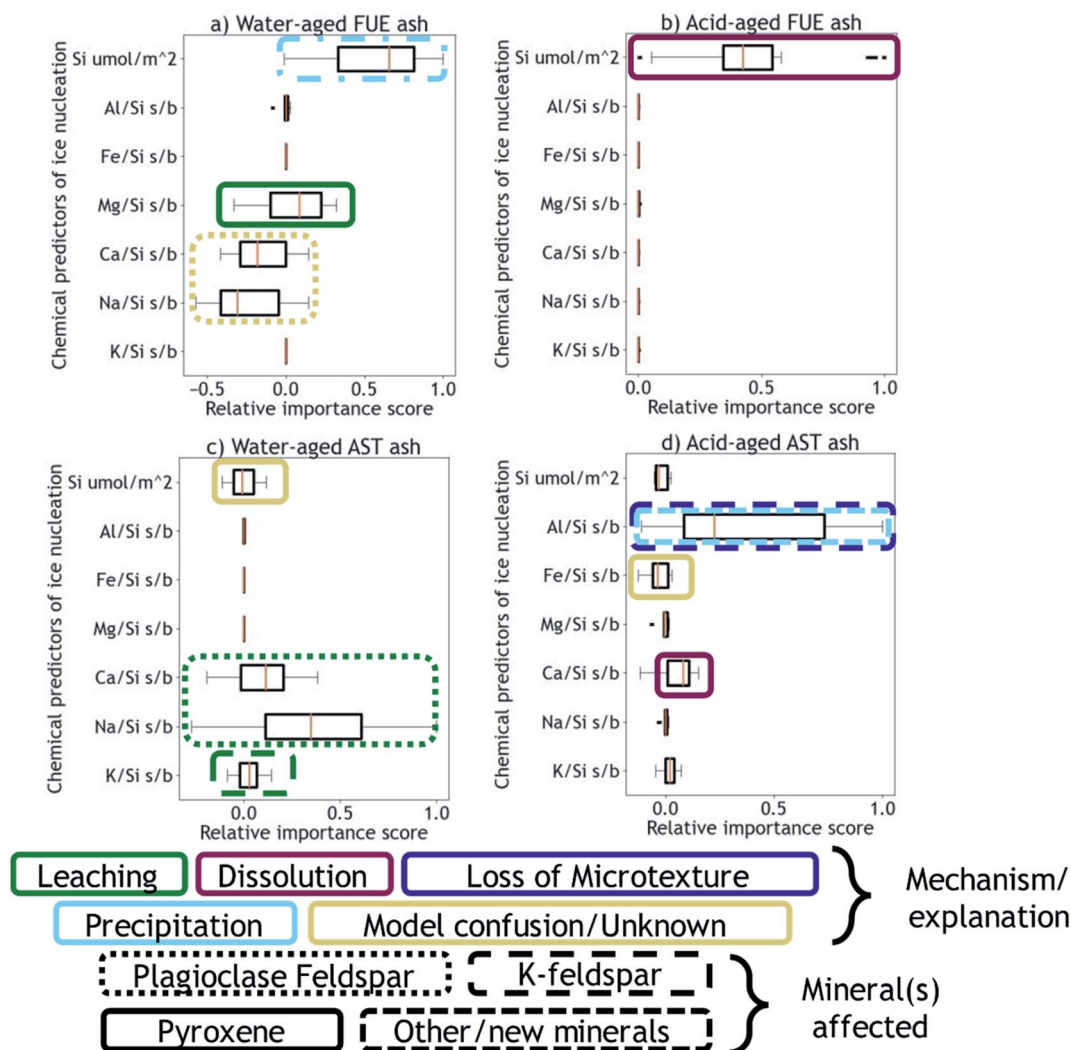
Fig. 3 Permutation importances of mean element signatures to the predictive model of INA for FUE ash aged in (a) \text{H}_2\text{O} (water-aged) or (b) \text{pH} 1.75 \text{H}_2\text{SO}_4 (acid-aged), and AST ash aged in (c) \text{H}_2\text{O} (water-aged) or (d) \text{pH} 1.75 \text{H}_2\text{SO}_4 (acid-aged). All values are scaled such that 1.0 represents the maximum positive importance in each dataset. The proposed reaction mechanisms and the mineral(s) affected are indicated by the annotations using the box color and box line style, respectively.
