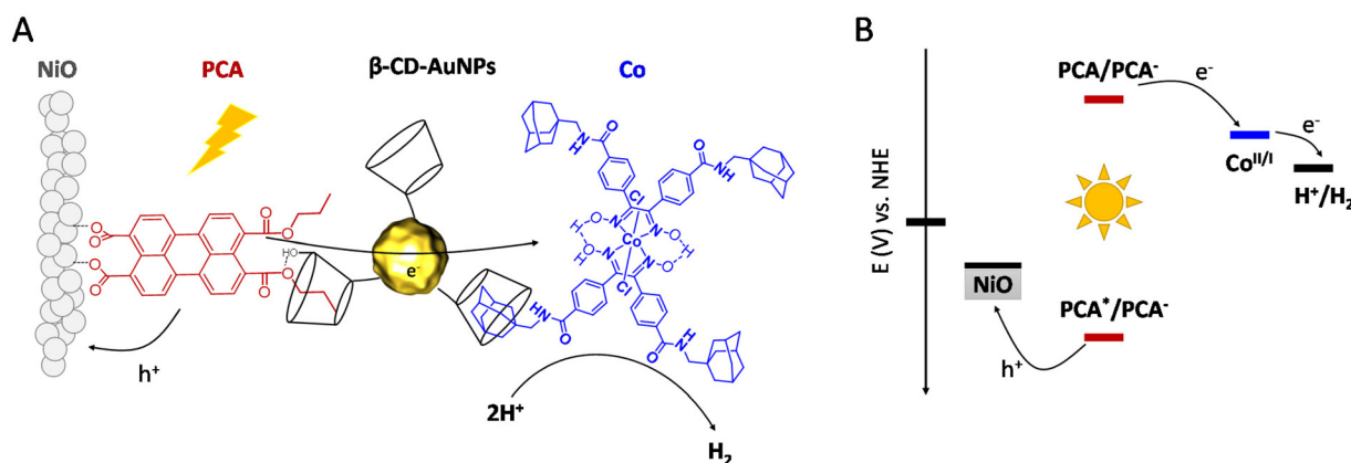
Fig. 1 (A) Representation of the PCA|β-CD-AuNPs|Co supramolecular assembly anchored onto a mesoporous NiO thin film, (B) energy diagram of the photocathode.
