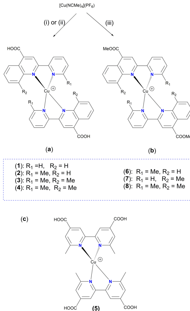
Scheme 2 Reaction scheme of the copper(i) cations of complexes 1–4 (a) and 6–8 (b); (i) pqca or 6'-Mepqca , DMSO; (ii) 8-Mepqca or 8,6'-Me 2 pqca , Me 2 CO; (iii) 6'-Mepqcame , 8-Mepqcame , 8,6'-Me 2 pqcame , CH 2 Cl 2 . (c) Molecular structure of 5 .
