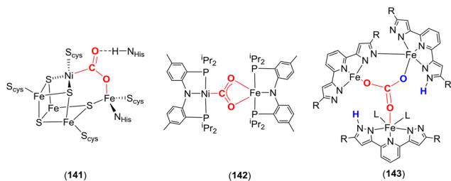
Fig. 5 Carbon monoxide dehydrogenase C-cluster active site ( 141 ) found in the enzyme and its biomimetic model ( 142 ). Trinuclear iron complex 143 is the functional model of carbonic anhydride.
