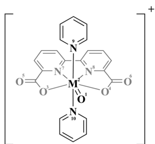
Fig. 3 [M V (bda)(py) 2 -O] + complexes included in the study (M = Fe or Ru) and numbering of atoms.
