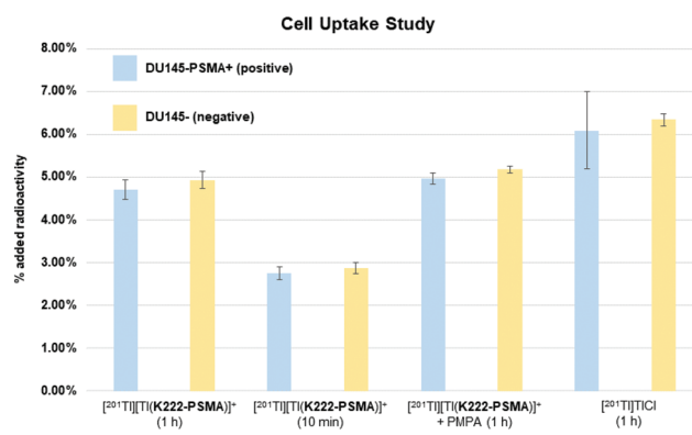
Fig. 6 Cell uptake study results for bioconjugate ^{201}\text{Tl}[\text{Tl}(\text{K222-PSMA})]^+ in PSMA-positive cell line, DU145-PSMA+ (positive) and the parental PSMA-negative DU145 cell line (negative) after 1 hour and 10 min incubation time (columns 1–4), in the presence of the PSMA inhibitor, 2-PMPA (2-(phosphonomethyl) pentane-1,5-dioic acid, columns 5 and 6). Columns 7 and 8 show the control experiment where positive and negative cells were incubated with “unchelated” ^{201}\text{Tl}[\text{Tl}(\text{i})]\text{Cl} for 1 h. Each experiment was conducted twice, values shown are the mean \pm standard deviation.
