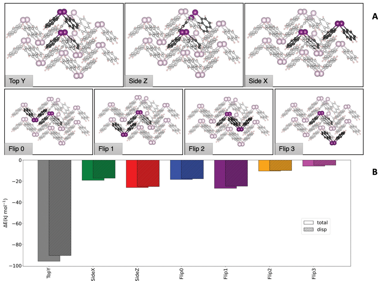
Fig. 5 (A) Dimers as cut from the 13-molecule cluster of \text{Bi}_2\text{Naph}_2 (1). Geometries are frozen at the experimental crystallographic ones. The highlighted molecules are the ones included in the calculations (see text) while the rest of the cluster is only shown to illustrate how the dimers were extracted. Colour code: C (black), Bi (purple), H (light pink). (B) Comparison between the different dimer formation energies at the PBE0/def2-TZVPP level of theory.
