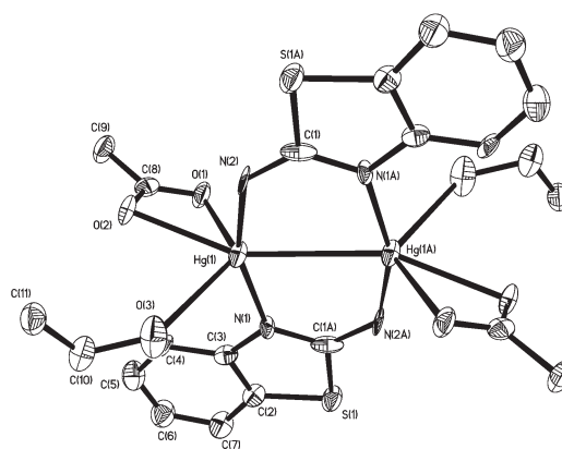
Fig. 1 Molecular structure of 3 . Thermal ellipsoids are displayed at 50% probability and hydrogen atoms omitted for clarity. Selected bond lengths (Å) and bond angles (°): Hg1–Hg1A 3.094(1), Hg1–N1 2.067(6), Hg1–N2 2.040(8), Hg1–O1 2.560(7), Hg1–O2 2.481(6), Hg1–O3 2.592(8), N1–C1A 1.348(11), N2–C1 1.286(10), C1–S1A 1.738(8); N1A–C1–N2 126.5(7), N1–Hg–N2 158.5(2), O1–Hg–O2 114.5(2), N1–Hg1–O3 91.1(2).
