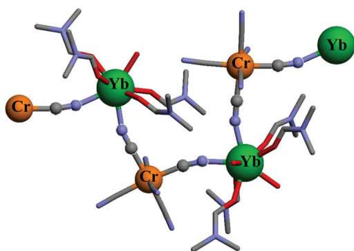
Fig. 1 Structure of part of the one-dimensional chain of \{[\text{Cr}(\text{CN})_6][\text{Yb}(\text{dmef})_4(\text{H}_2\text{O})_2] \cdot \text{H}_2\text{O}\}_\infty highlighting the Cr–CN–Yb bridges. 33 Color code: C = grey, N = blue, O = red, Cr = orange, Yb = green.
