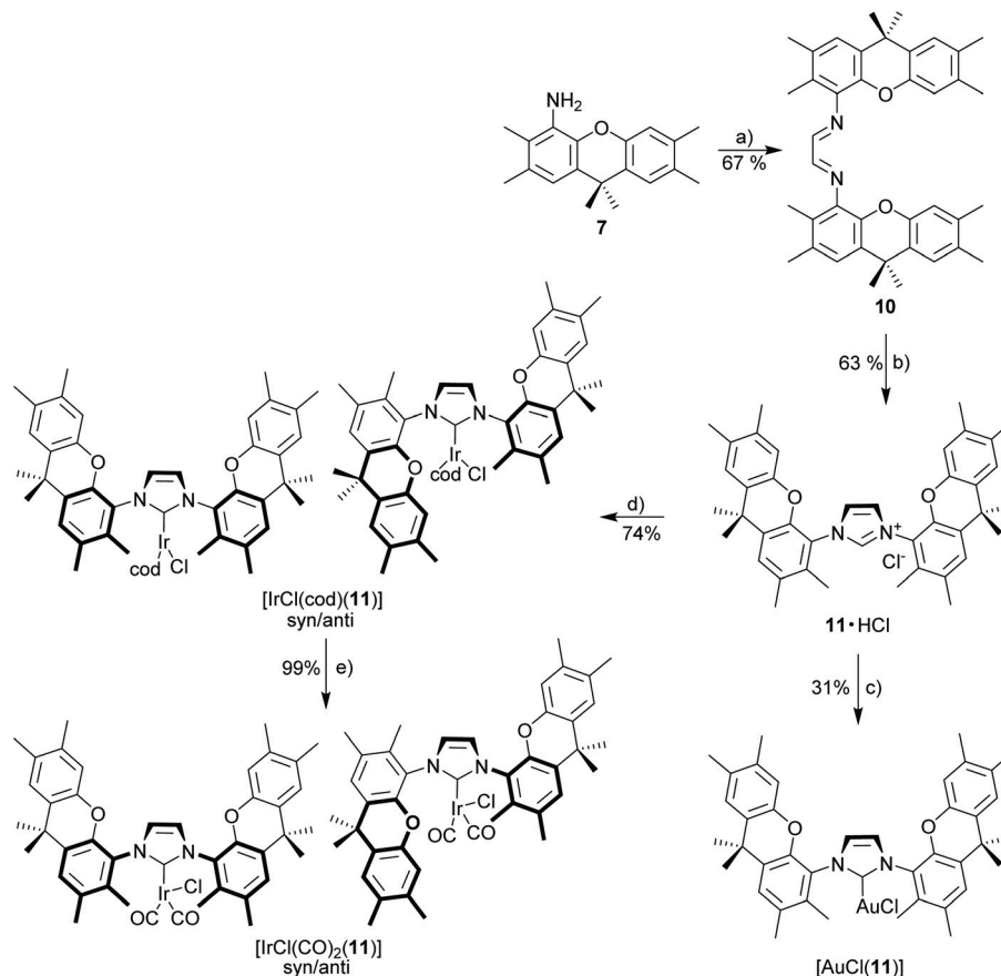
Scheme 4 Synthesis of imidazolium salt 11·HCl and derived metal complexes. Reagents and conditions: (a) glyoxal, p TsOH, EtOH, 50 °C; (b) paraformaldehyde, \text{Me}_3\text{SiCl} , EtOAc, 70 °C, 24 h; (c) [\text{AuCl}(\text{SMe}_2)]_2 , \text{K}_2\text{CO}_3 , acetone, 50 °C; (d) [\text{IrCl}(\text{cod})]_2 , \text{K}_2\text{CO}_3 , acetone, 50 °C; (e) CO, 0 °C, 30 min, \text{CH}_2\text{Cl}_2 .
