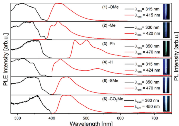
Fig. 5 Excitation and emission spectra of compounds 1–6 in the solid state at 77 K. The PLE/PL spectra were excited/recorded at the values given on the right side of the graph. Photographs of the PL samples: UV lamp ( \lambda_{exc} = 256 nm).
