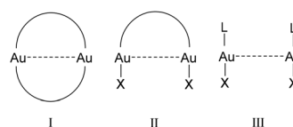
Fig. 1 Classification of closed-shell aurophilic interactions into fully-supported (I), semi-supported (II) and unsupported (III).
