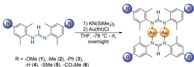
Scheme 4 Synthesis of gold complexes 1–6.
