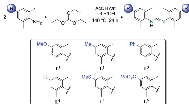
Scheme 2 Synthesis of amidine ligands L 1 – L 6 via the ethanol condensation reaction.
