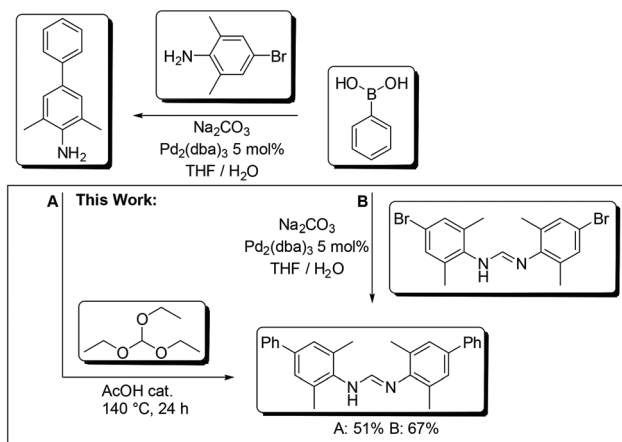
Scheme 3 Synthesis routes of L 3 with Suzuki coupling before (left) and after (right) amidine formation.
