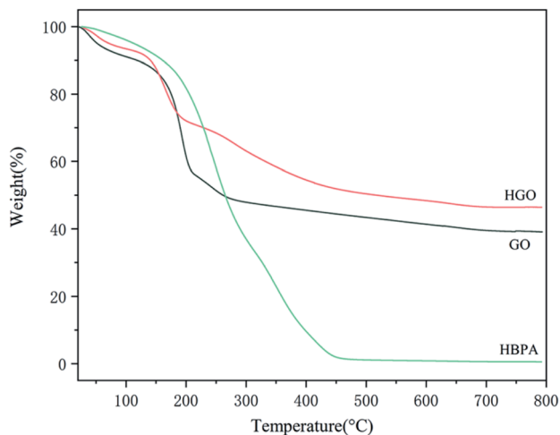
Fig. 6 TGA spectra of GO, HGO, and HBPA.
