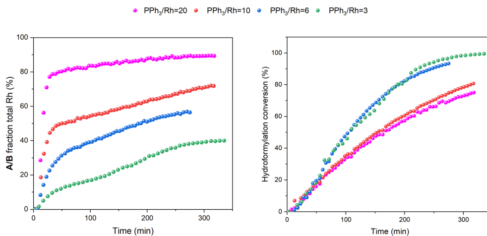
Fig. 5 Amount of A/B detected by quantitative 1 H FlowNMR spectroscopy during hydroformylation of 1-hexene under 12 bar of CO/H 2 (1 : 1) at 50 °C catalysed by [Rh(acac)(CO) 2 ] = 2.5 mM and [PPh 3 ] = 7.5, 15, 25 and 50 mM in 22.4 mL of non-deuterated toluene versus conversion over time.
