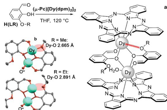
Scheme 39 (a) Transformation of inverted sandwich (\mu\text{-Pc})[\text{Dy}(\text{dpm})_2]_2 into a triple-decker mixed ligand complex (\mu\text{-LR})_2\text{Dy}_2(\text{Pc})_2(\text{H}_2\text{O}) upon interaction with 3-alkoxysalicylic aldehydes, \text{H}(\text{LR}) , \text{R} = \text{OMe} , \text{OEt} . (b) Structure of the middle layers formed by deprotonated ligands \text{LR}^- , coordinated to dysprosium ions (CCDC MESMIJ, \text{R} = \text{Me} and MESMOP, \text{R} = \text{Et} ). 201
