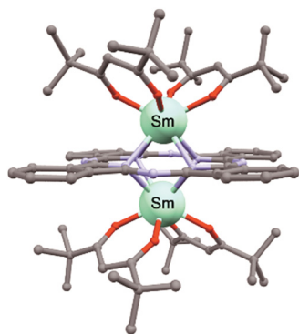
Fig. 8 X-ray structure of (\mu\text{-Pc})[\text{Sm}(\text{dpm})_2]_2 (CCDC CALWIV). 194 Solvate molecules and hydrogen atoms are not shown.
