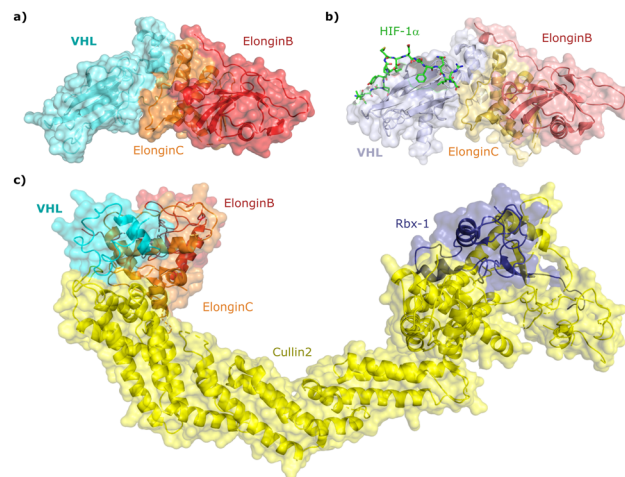
Fig. 2 Crystal structure of VCB (PDB 1VCB) (a), 40 cocystal structure of HIF-1 \alpha peptide bound to VCB (PDB 1LM8) (b), 41 and structure of the full length VCB-Cul2-Rbx1 multidomain complex (PDB 5N4W) (c). 42
