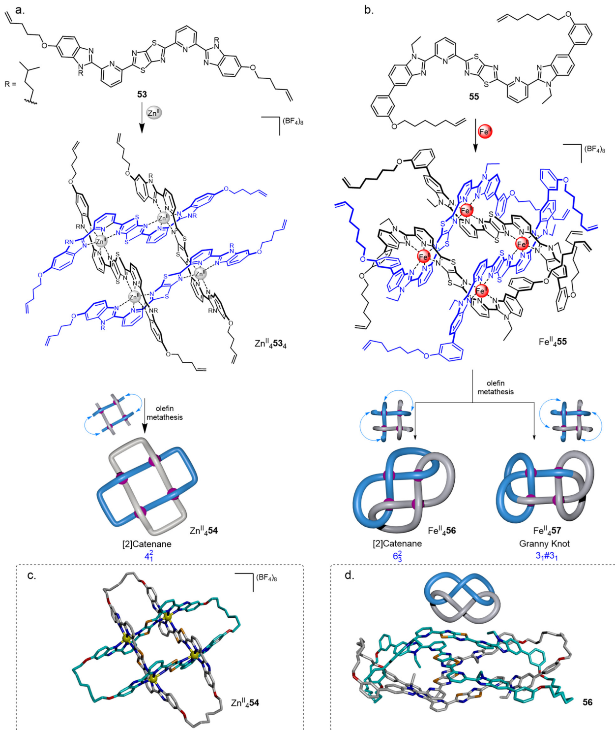
Fig. 20 Synthesis of 2 × 2 interwoven molecular grids and their closures by olefin metathesis to generate (a) Solomon link 54 , 14 or (b) 6 3 link 56 and granny knot 57 , 15 X-ray crystal structures of (c) Zn II 4 54 and (d) demetallated link 56 .
