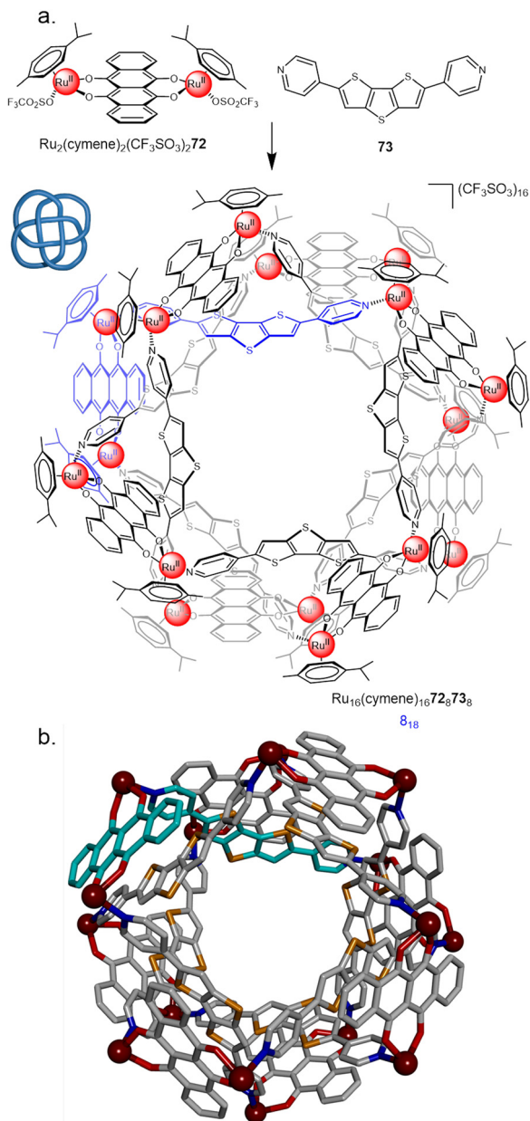
Fig. 25 (a) Synthesis of \delta_{18} metalla-knot \text{Ru}_{16}(\text{p-cymene})_{16}\text{72}_8\text{73}_8 . (b) X-ray crystal structure of the \delta_{18} metalla-knot with p -cymene ligands omitted for clarity. 100
