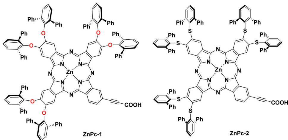
Fig. 67 Molecular structures of phthalocyanine sensitizers ZnPc-1 and ZnPc-2.
