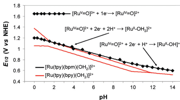
Fig. 120 Plots of E 1/2 (V vs. NHE) vs. pH for the Ru(v/iv) and Ru(iv/iii) redox couples of [Ru(tpy)(bpm)(OH 2 )] 2+ and for the Ru(III/II) and Ru(III/II) redox couples of [Ru(tpy)(bpy)(OH 2 )] 2+ in aqueous solution (I) 0.1 M; (T) 298 K; glassy carbon working electrode). Reprinted with permission from ref. 1479 Copyright 2008. American Chemical Society.
