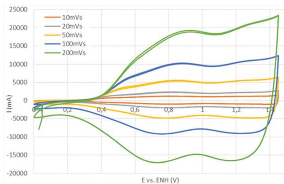
Fig. 101 (left) SEM micrographs of unsupported \text{IrO}_2 nanoparticles used at the anode of PEM water electrolysis cells. (right) In situ cyclic voltammograms recorded on \text{IrO}_2 at the anode of a PEM water electrolysis cell, at different scan rates. Reproduced with permission from ref. 116. Copyright Elsevier 2016.
