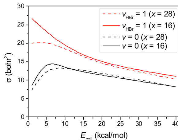
Fig. 3 Initial distance dependence of the integral cross sections for the \text{HBr}(v_{\text{HBr}} = 0, 1) + \text{C}_2\text{H}_5(v = 0) \rightarrow \text{Br} + \text{C}_2\text{H}_6 reactions as a function of collision energy, where the initial distance between the center of mass of \text{HBr} and the center of mass of \text{C}_2\text{H}_5 is (x^2 + b^2)^{1/2} , with x = 16 and 28 bohr.
