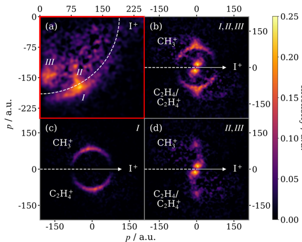
Fig. 6 (a) Momentum distribution of I^+ covariant with CH_3^+ , produced from the three-body breakup of 2-IP 2+/3+ . The red box around this panel is to highlight the different scale for the momentum axes, and the different frame in which these data are presented. The three dissociation channels are as follows: (I) sequential three-body breakup of 2-IP 3+ , (II) concerted three-body breakup of 2-IP 3+ , (III) three-body breakup of 2-IP 2+ . (b) Newton diagram for the same process, displaying the CH_3^+ momentum in the COM frame of the charged propyl intermediate. Filtering based on the absolute I^+ momentum has been used to isolate (c) the sequential breakup channel of 2-IP 3+ ( 190 < p_{I^+} < 225 a.u.) from (d) the signal due to concerted breakup of 2-IP 3+ as well as three-body breakup of 2-IP 2+ ( 120 < p_{I^+} < 190 a.u.).
