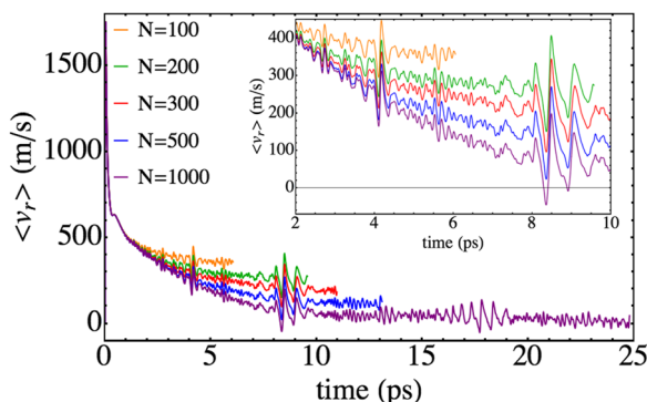
Fig. 5 Time evolution of the mean value of the Br–Br relative velocity for different nanodroplet sizes.
