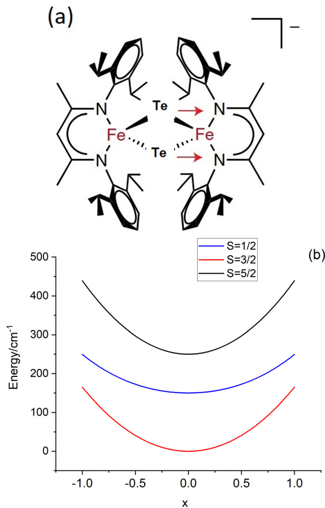
Fig. 4 (a) Representation of the anion [\text{L}_2\text{Fe}_{24}\text{Te}_2]^- , the red arrows depict the asymmetric (symmetry breaking) mode ( q ); (b) adiabatic ground state ( S = 3/2 ) and two lowest ( S = 1/2 , S = 5/2 ) excited states along q ; The curves were plotted taking the values of J = -200 \text{ cm}^{-1} and B = 750 \text{ cm}^{-1} (from ref. 10) and the vibronic coupling energy \lambda = 480 \text{ cm}^{-1} (see Table 7).
