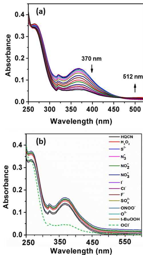
Fig. 2 (a) UV-vis spectra of HQCN ( 10\ \mu\text{M} in \text{CH}_3\text{OH}-\text{H}_2\text{O} ; 1/4, v/v in the presence of HEPES buffer (10 mM) solution at pH = 7.2) upon the gradual addition of \text{OCl}^- (0 to 5 equivalents). Ratiometric spectra of HQCN were observed after the addition of \text{OCl}^- . The absorption peak of HQCN at 370 nm gradually decreased and the peak at 512 nm gradually increased after the addition of \text{OCl}^- with an isosbestic point at 462 nm. (b) UV-vis spectra of HQCN ( 10\ \mu\text{M} in \text{CH}_3\text{OH}-\text{H}_2\text{O} ; 1/4, v/v in the presence of HEPES buffer (10 mM) solution at pH = 7.2) upon addition of different guest analytes (0 to 5 equivalents). Apart from \text{OCl}^- , no significant change was observed upon the addition of the other guest analytes.
