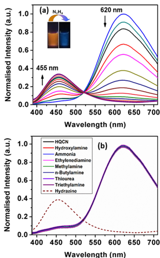
Fig. 3 (a) Fluorescence emission spectra of HQCN ( 10\ \mu\text{M} in \text{CH}_3\text{OH}-\text{H}_2\text{O} ; 1/4, v/v in the presence of HEPES buffer (10 mM) solution at pH = 7.2) upon the gradual addition of \text{N}_2\text{H}_4 (0 to 5 equivalents) where the \lambda excitation was 370 nm. Ratiometric spectra of HQCN were observed after the addition of \text{N}_2\text{H}_4 . The emission peak of HQCN at 620 nm gradually decreased and the peak at 455 nm gradually increased after the addition of hydrazine with an isoemissive point at 520 nm, inset shows the visible emission of HQCN in the absence and presence of 2 equivalents of hydrazine upon irradiation under UV light. (b) Fluorescence emission spectra of HQCN ( 10\ \mu\text{M} in \text{CH}_3\text{OH}-\text{H}_2\text{O} ; 1/4, v/v in the presence of HEPES buffer (10 mM) solution at pH = 7.2) after the addition of different guest analytes (0 to 5 equivalents). Apart from hydrazine, no significant change was observed for other guest amines.
